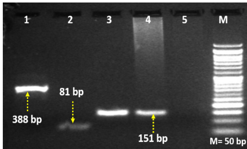
Figure 2. Amplification of CCL8, CXCL10 and GAPDH gene. Lane 1: CCL8; Lane 2: GAPDH; Lane 3-4: CXCL10
