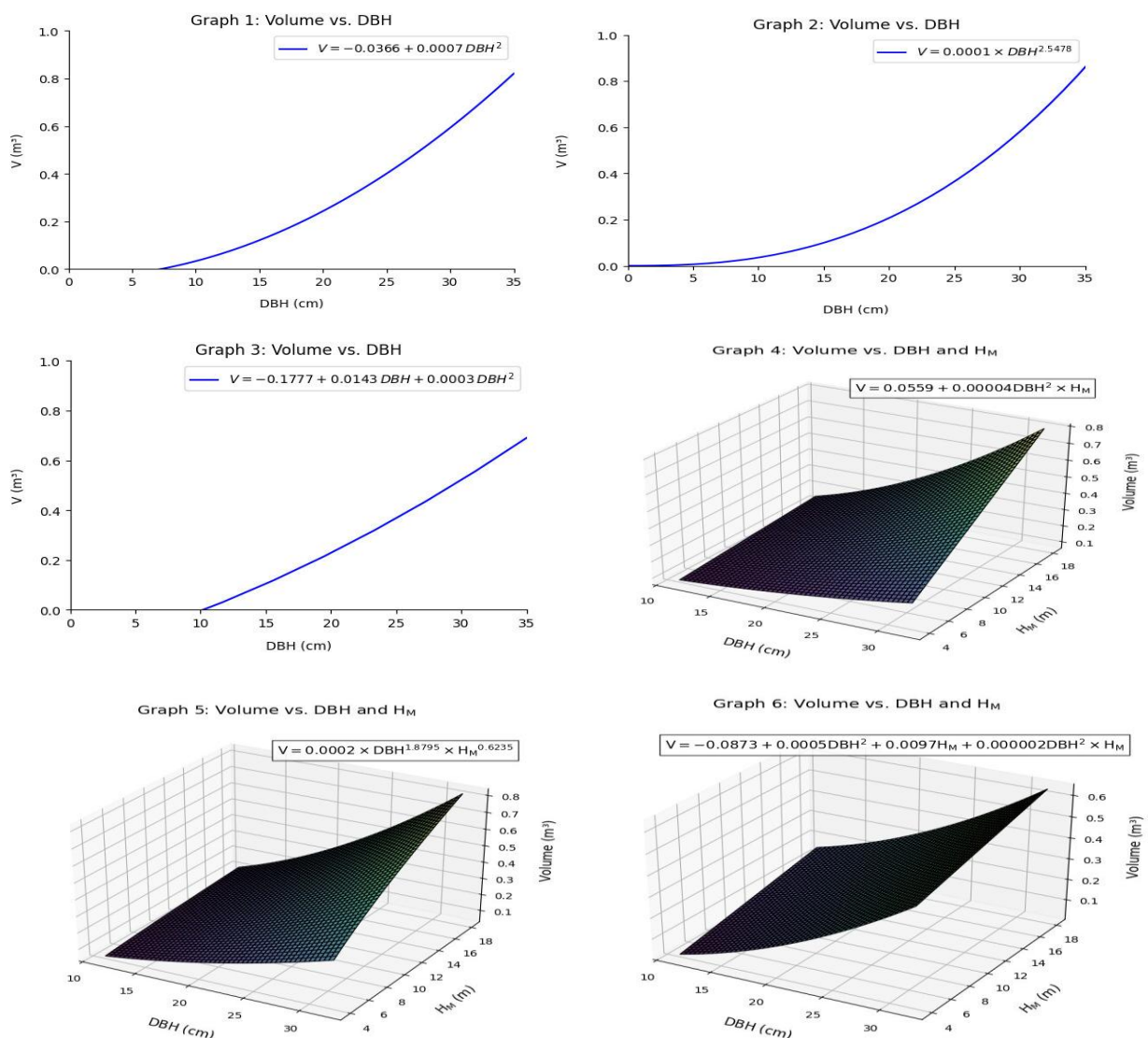
Figure 6 Relationship between DBH, merchantable height and merchantable volume from equations 1- 6
